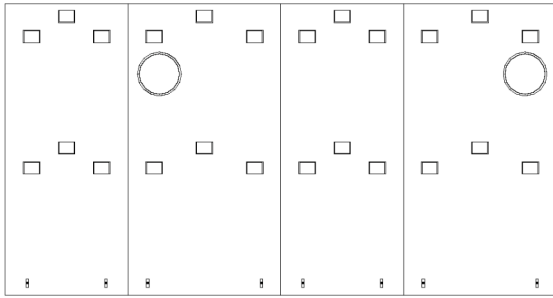
Casing (unfolded)
